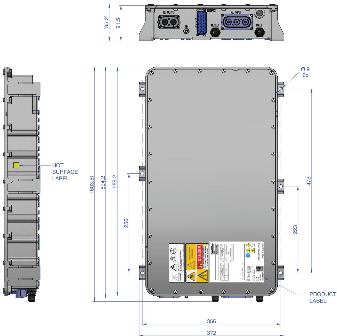
Figure 7. Mechanical Drawing
