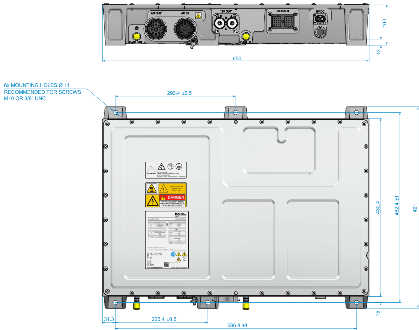
Figure 2. Mechanical Drawing
