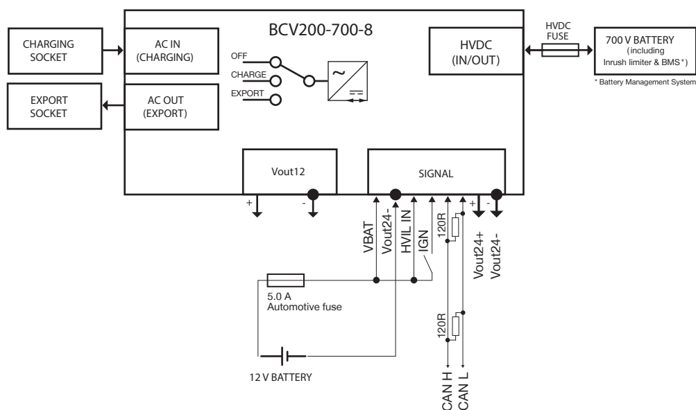
Figure 1. Schematic diagram
