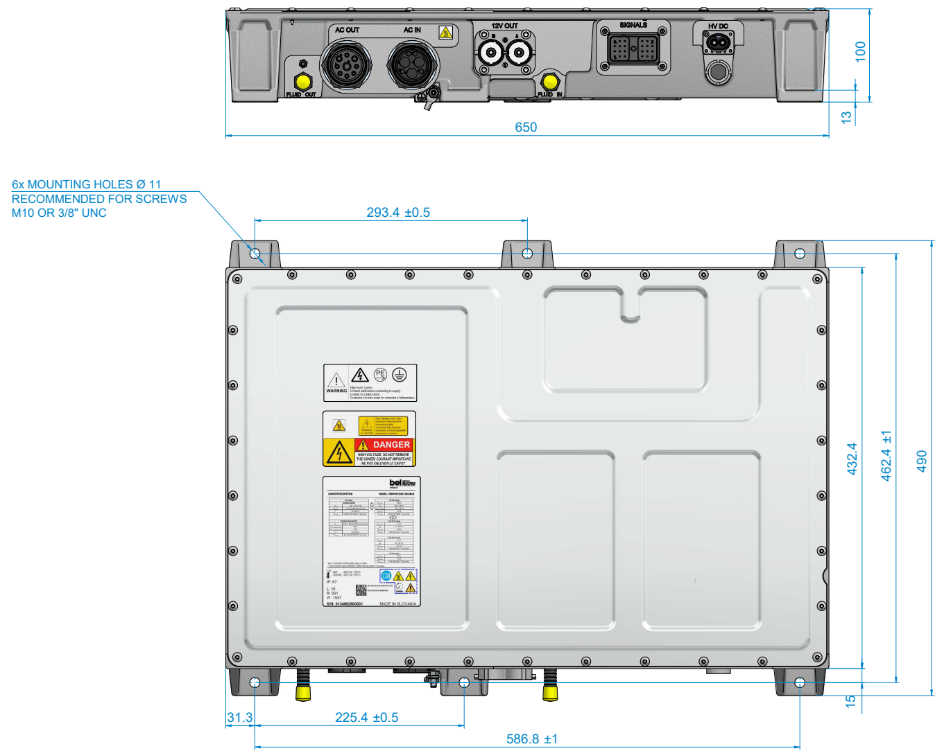
Figure 2. Mechanical Drawing
