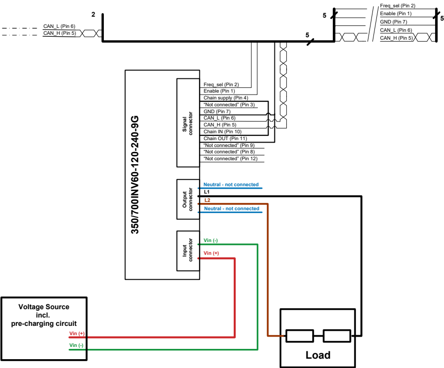
Figure 2b. Wiring setup for single operation of 350/700INV60-120-240-9G, 1x 240 VAC, 1x 6 kVA, L1 to L2 (N must not be connected)
