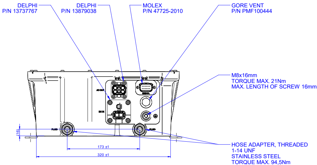
Figure 5. Front view
