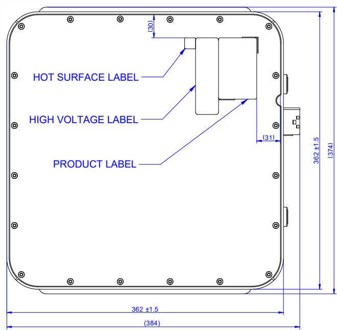
Figure 7. Top view
