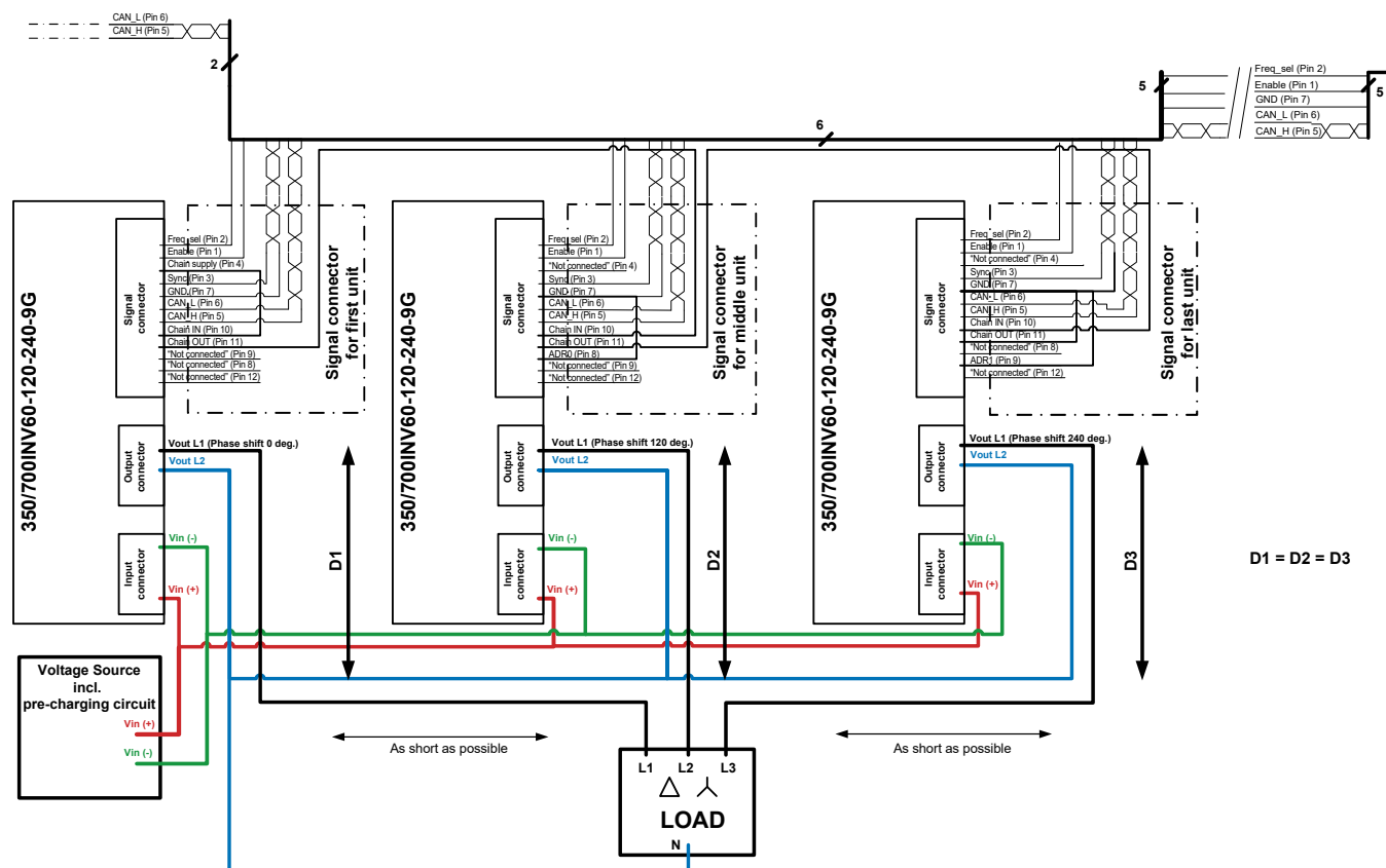
Figure 3a. Case A: Wiring setup for 3-phase operation, one load 3x 400 VAC / 25 A for 350/700INV60-120-240-9G
