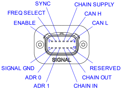
Signal Connector
