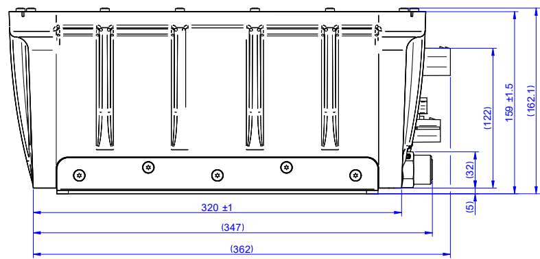
Figure 6. Side view
