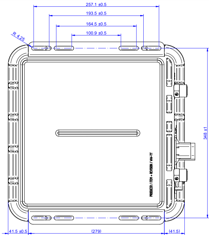
Figure 8. Bottom view
