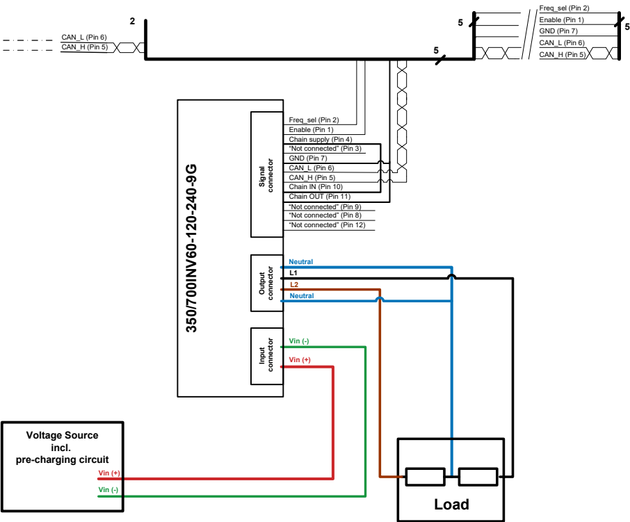
Figure 2a. Wiring setup for single operation of 350/700INV60-120-240-9G, 2x 120 VAC, 2x 3 kVA, L to N
