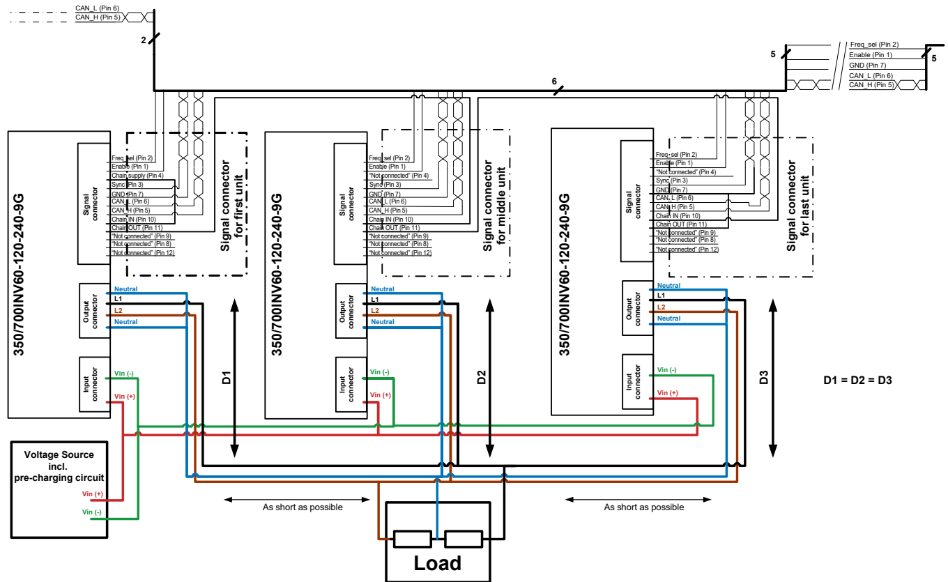
Figure 1. Wiring setup for parallel operation 350/700INV60-120-240-9G
