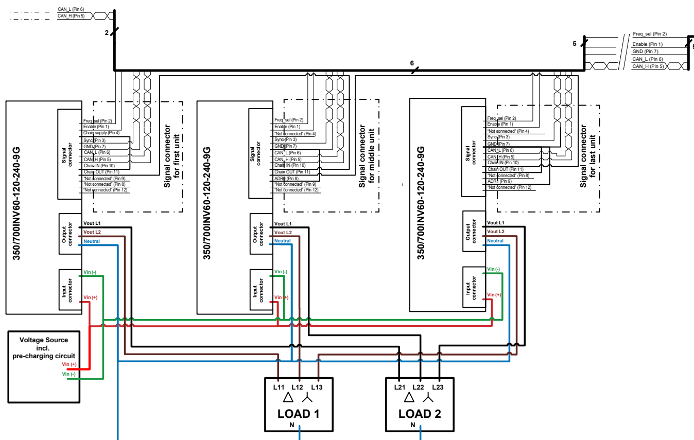
Figure 3b. Case B: Wiring setup for 3-phase operation, two independent loads 3x 208 VAC / 25 A for 350/700INV60-120-240-9G
