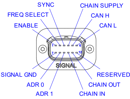
Signal Connector
