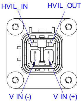
DC Input Connector
