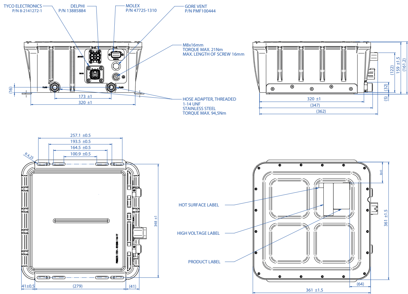
Figure 5. Front view
