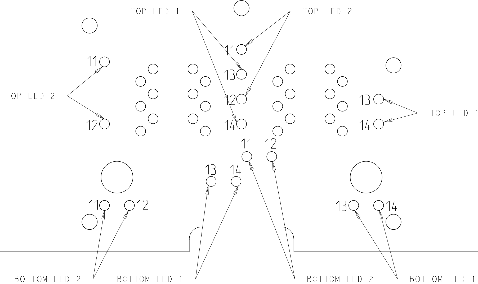
LED HOLE DESIGNATIONS VIEWED FROM COMPONENT SIDE
